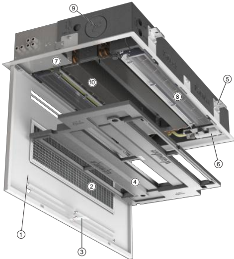
KaDeck at a glance (example shows two-sided air discharge, wet cooling)
